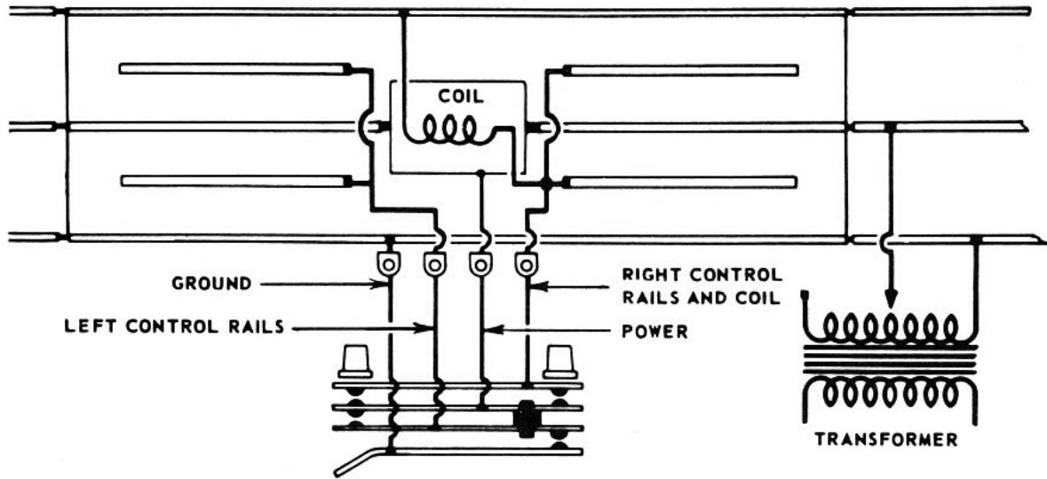
Figure 6 - Schematic Wiring Diagram of Remote Control Set Type UCS
